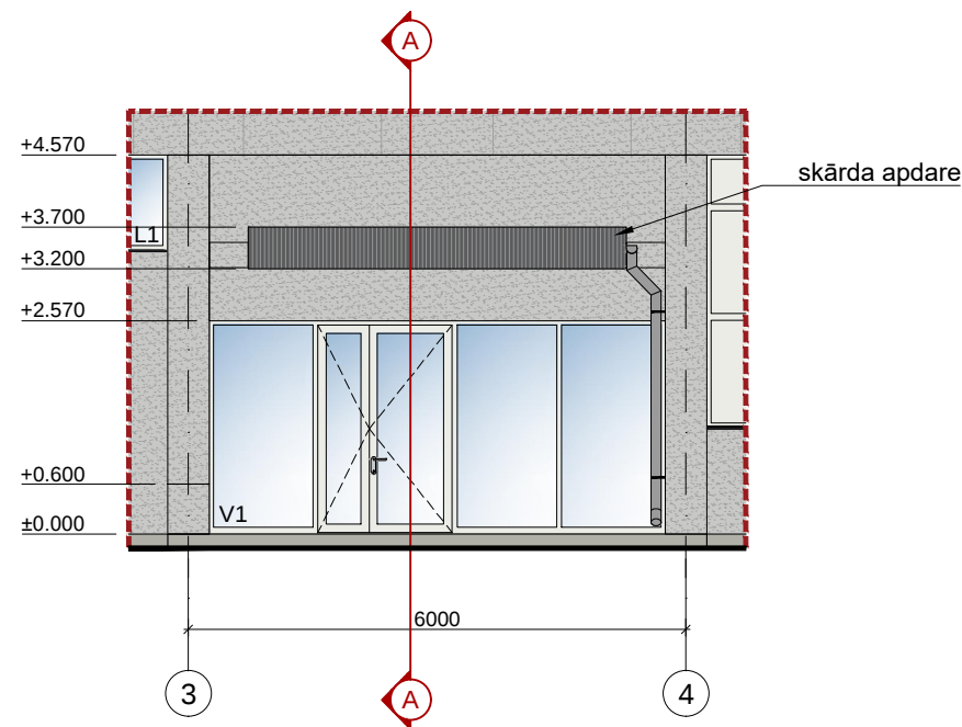
FASĀDES 1-10 FRAGMENTS (M1:100)
