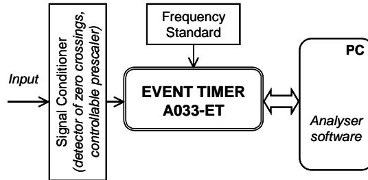
Fig. 2. Simplified block diagram of Jitter Analyzer.
