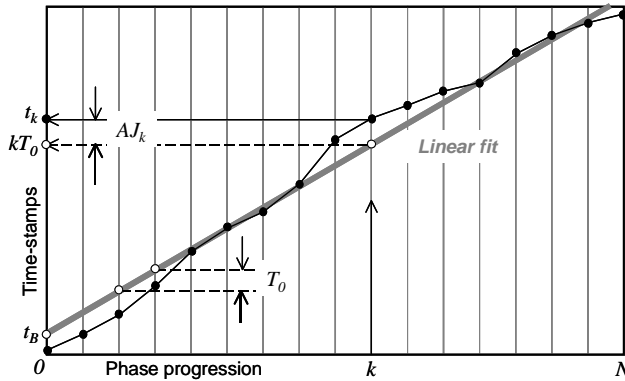
Fig. 1. Principle of jitter measurement through event timing.
