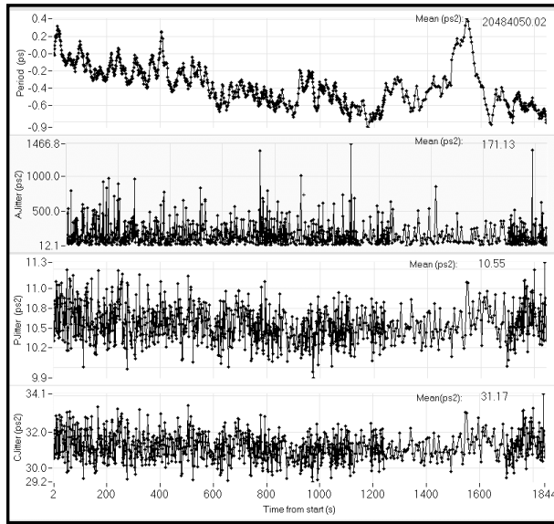
Fig. 4. Generalized characteristics of crystal clock generator jitter from cycle-to-cycle. From top to bottom: signal period deviation, squared RMS deviations of A-jitter, P-jitter and C-jitter respectively. Observation time: 30 min.
