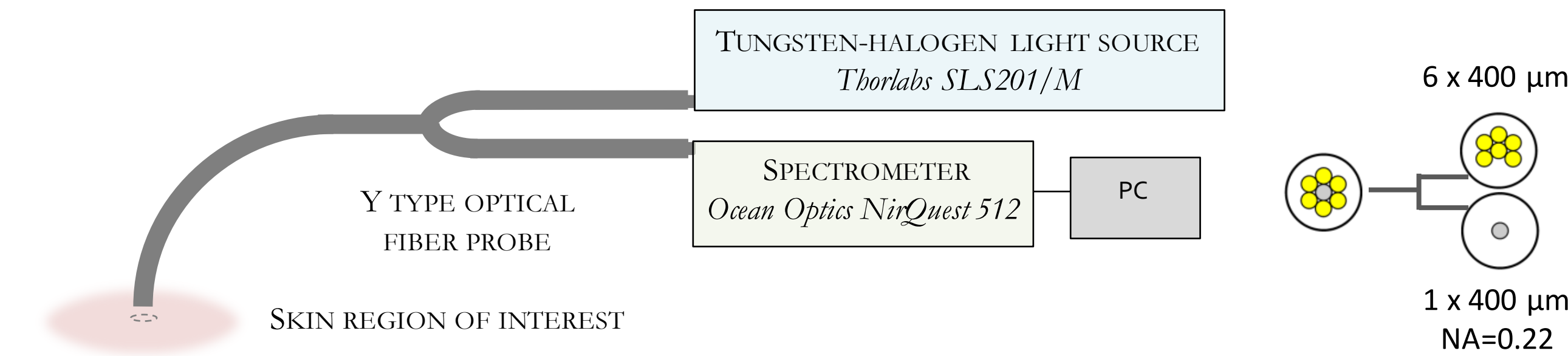
Fig.3 EXPERIMENTAL SETUP
