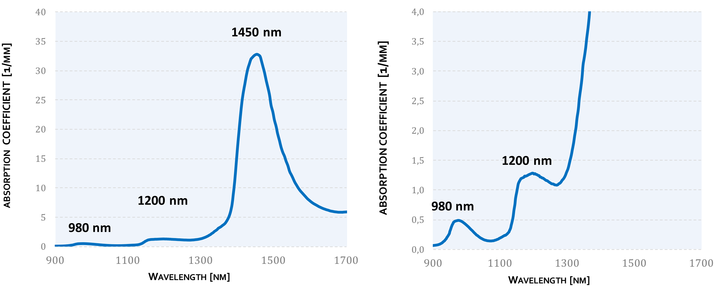
Fig.5 ABSORPTION SPECTRUM OF WATER [7]
